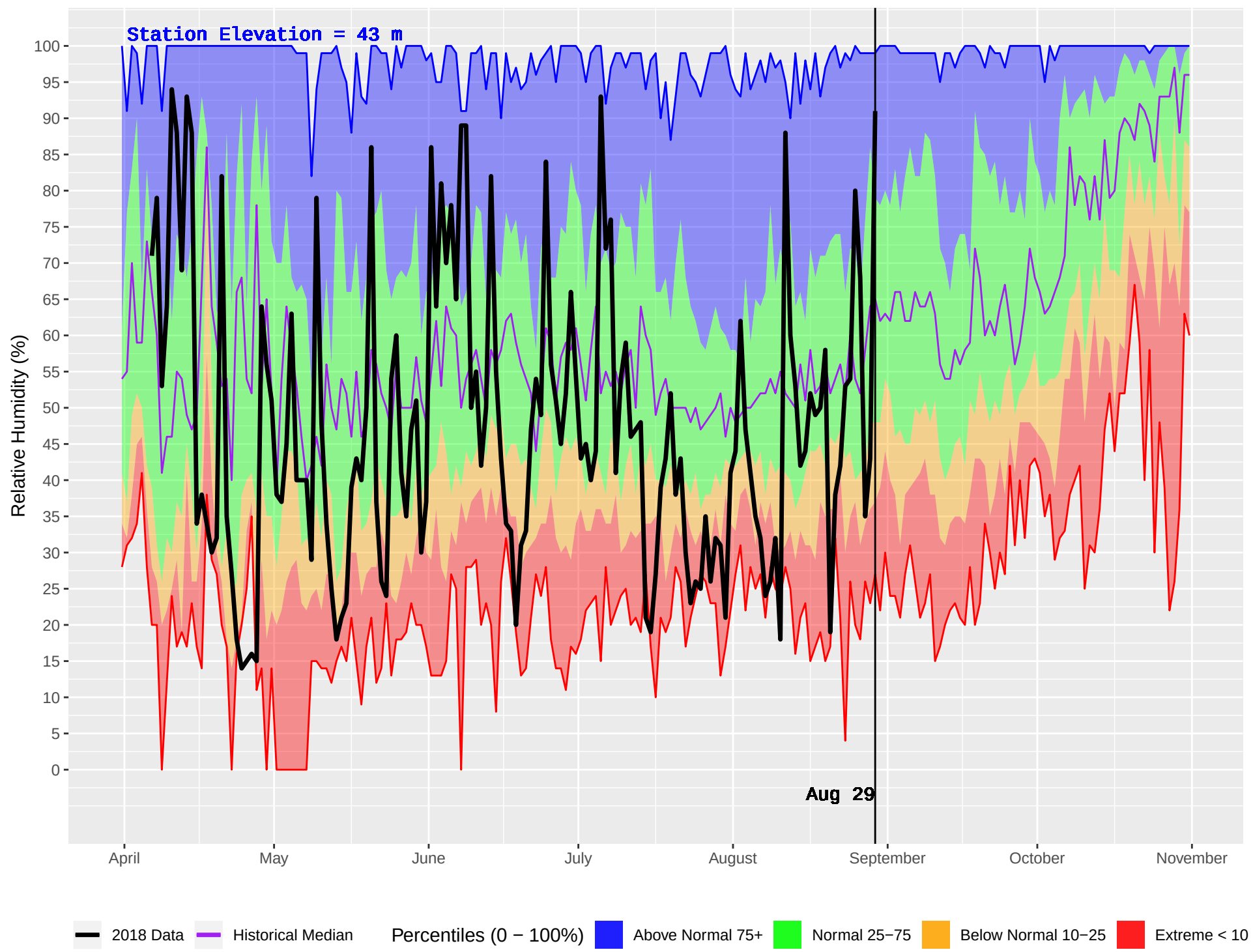
TOBA CAMP (75) : Historical (1970–2016) and Current (2018) Daily Relative Humidity
