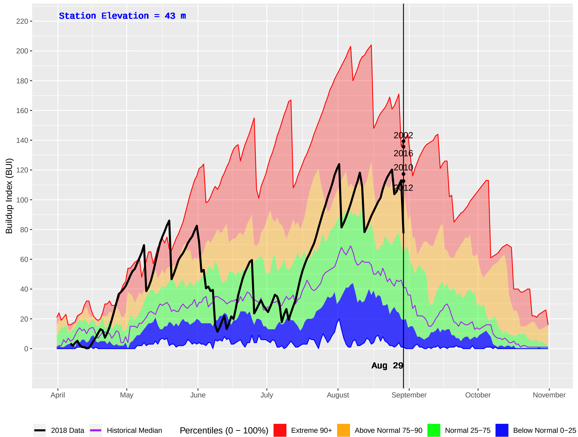
TOBA CAMP (75) : Historical (1970–2016) and Current (2018) Daily Buildup Index (BUI)
