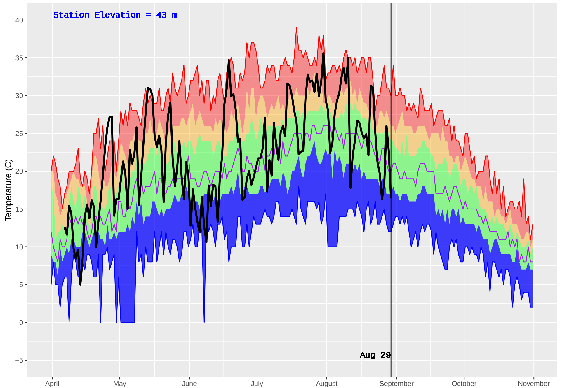
TOBA CAMP (75) : Historical (1970–2016) and Current (2018) Daily Temperature
