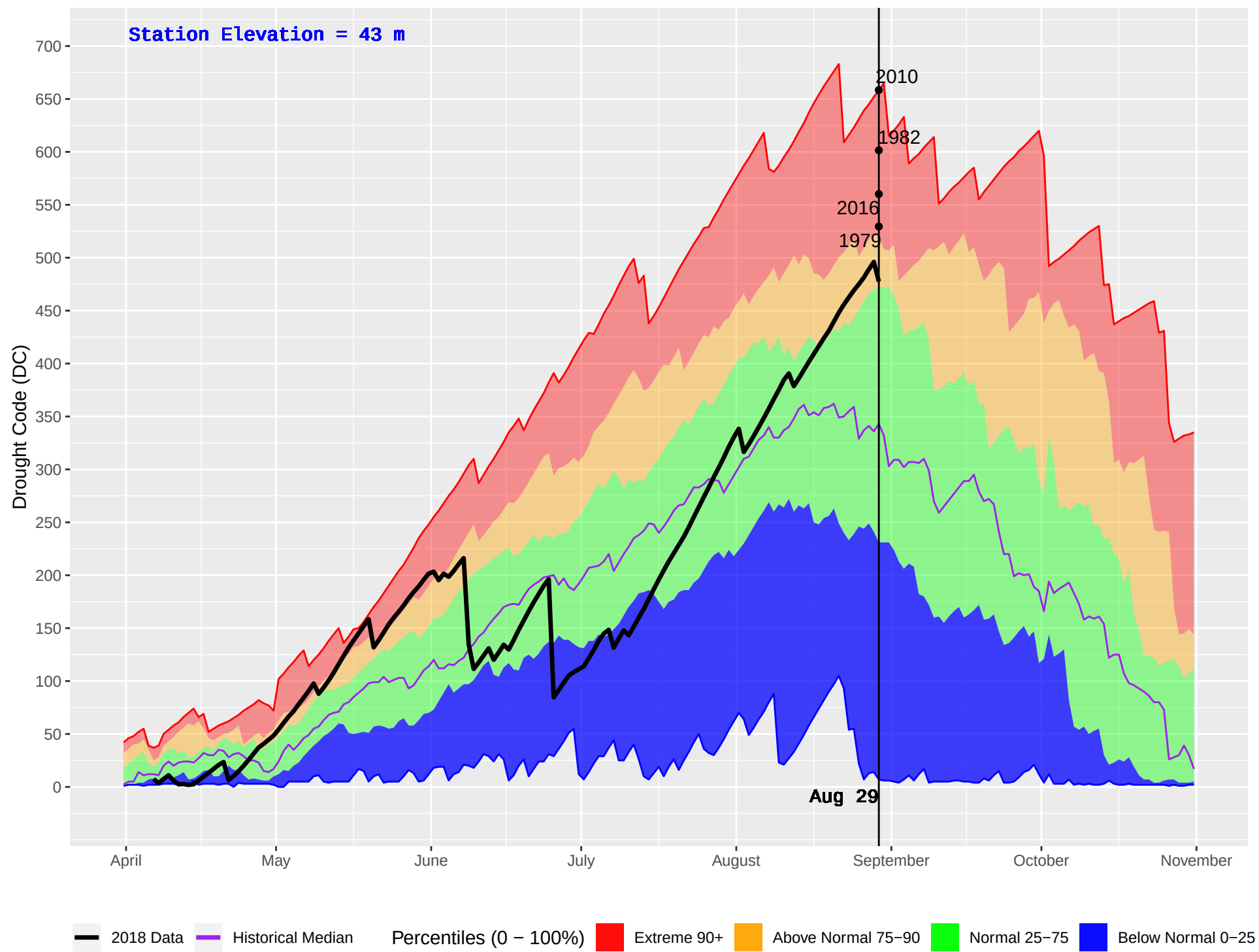
TOBA CAMP (75) : Historical (1970–2016) and Current (2018) Daily Drought Code (DC)
