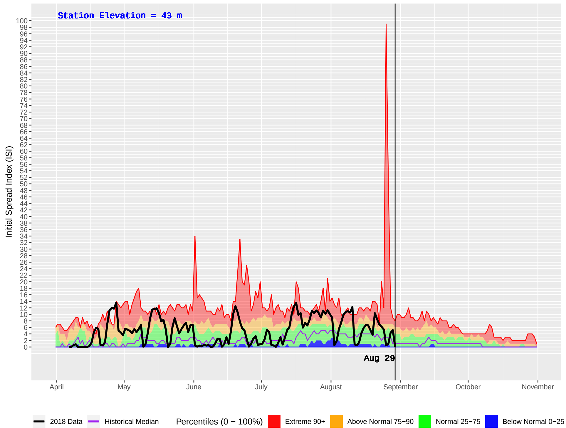
TOBA CAMP (75) : Historical (1970–2016) and Current (2018) Daily Initial Spread Index (ISI)
