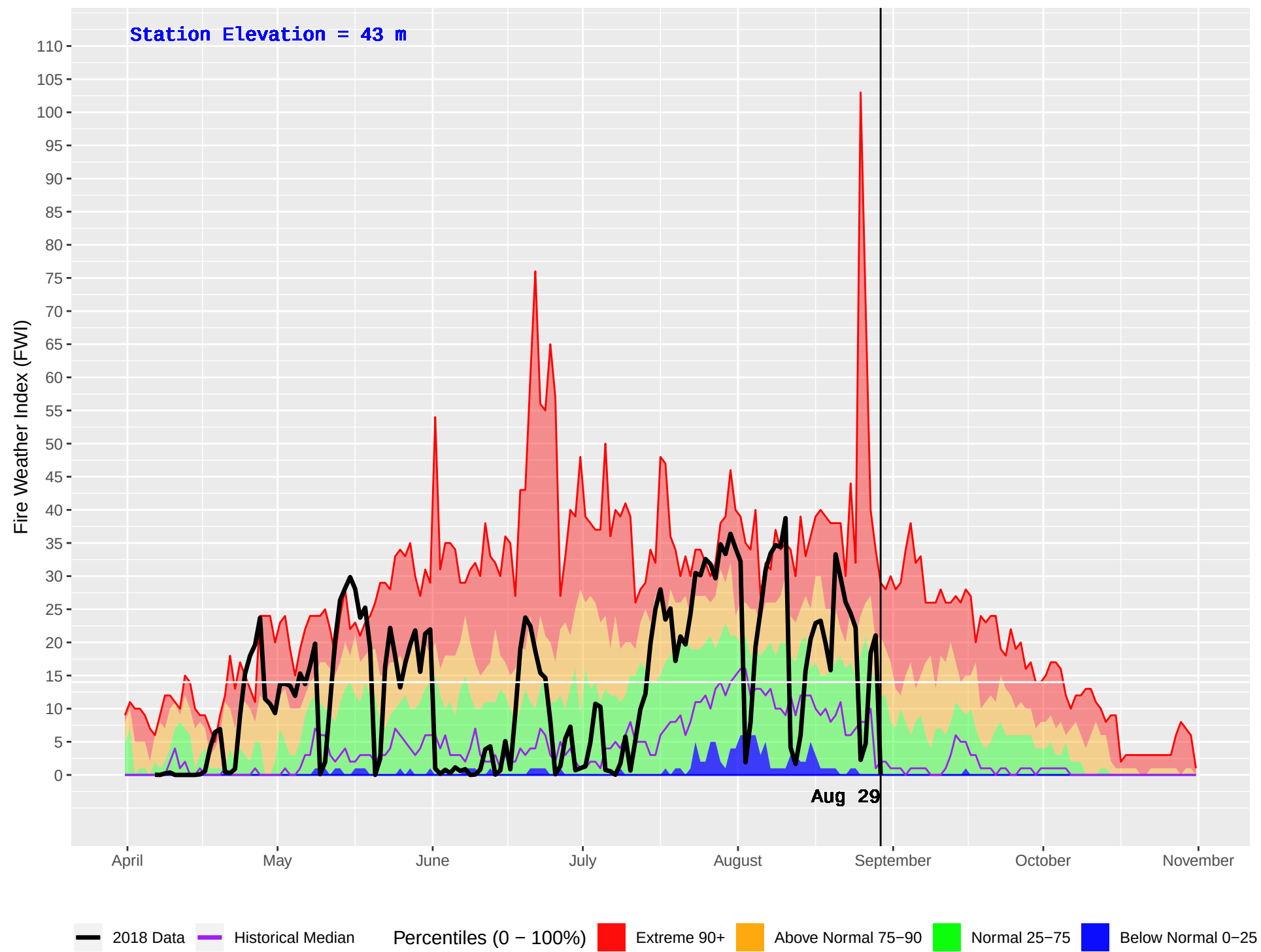
TOBA CAMP (75) : Historical (1970–2016) and Current (2018) Daily Fire Weather Index (FWI)
