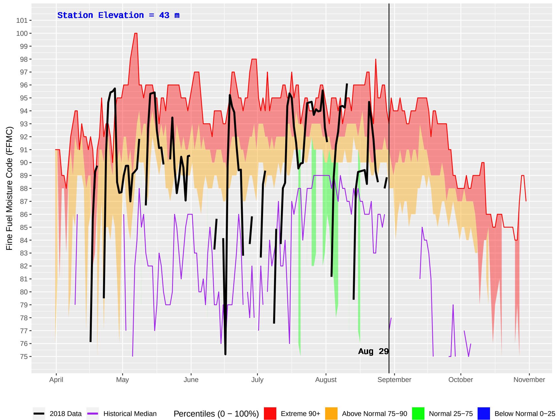
TOBA CAMP (75) : Historical (1970–2016) and Current (2018) Daily Fine Fuel Moisture Code (FFMC)
