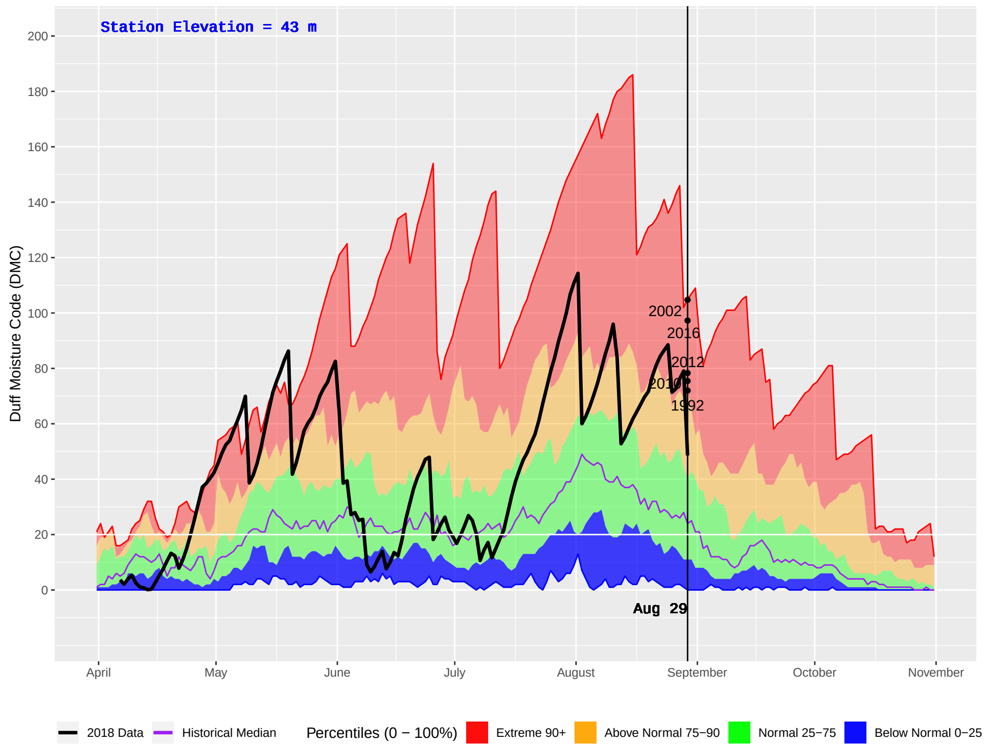
TOBA CAMP (75) : Historical (1970–2016) and Current (2018) Daily Duff Moisture Code (DMC)
